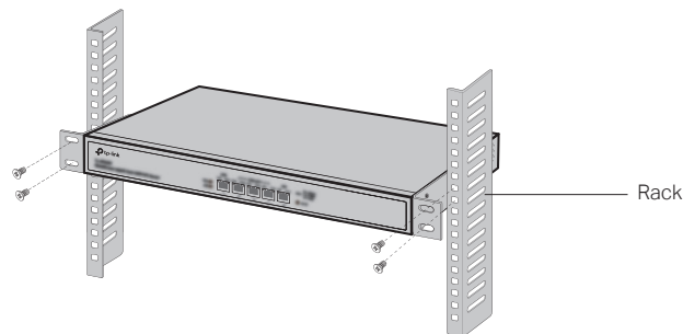
Figure 2-3 Rack Installation
