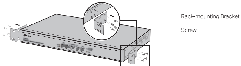
Figure 2-2 Bracket Installation
